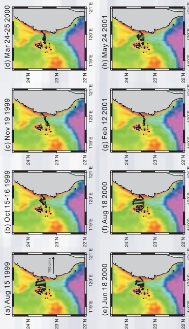
Fig. 5 Horizontal distribution of the depth-averaged subtidal flow.
