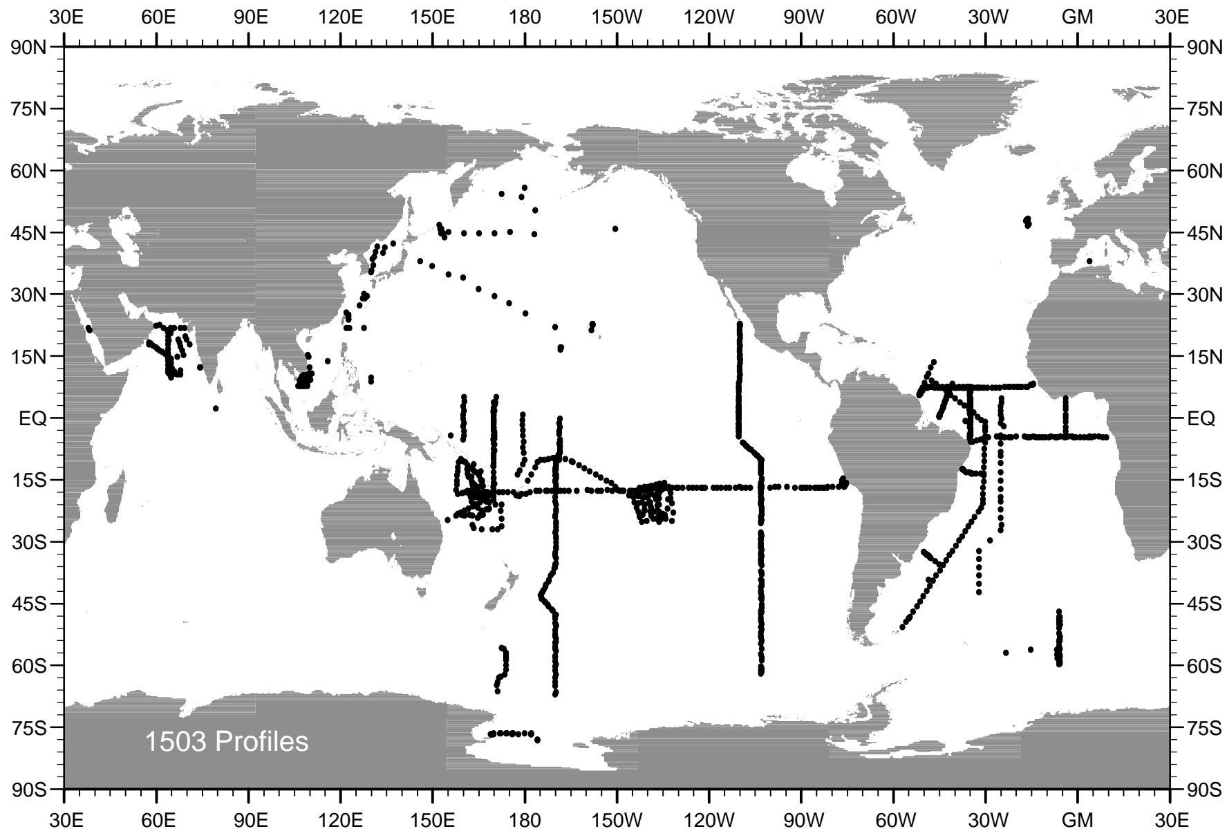
Distribution of Alkalinity, pH, and TCO2 Data
