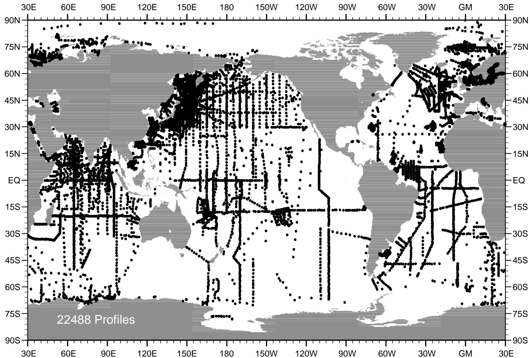
Distribution of Alkalinity Data
